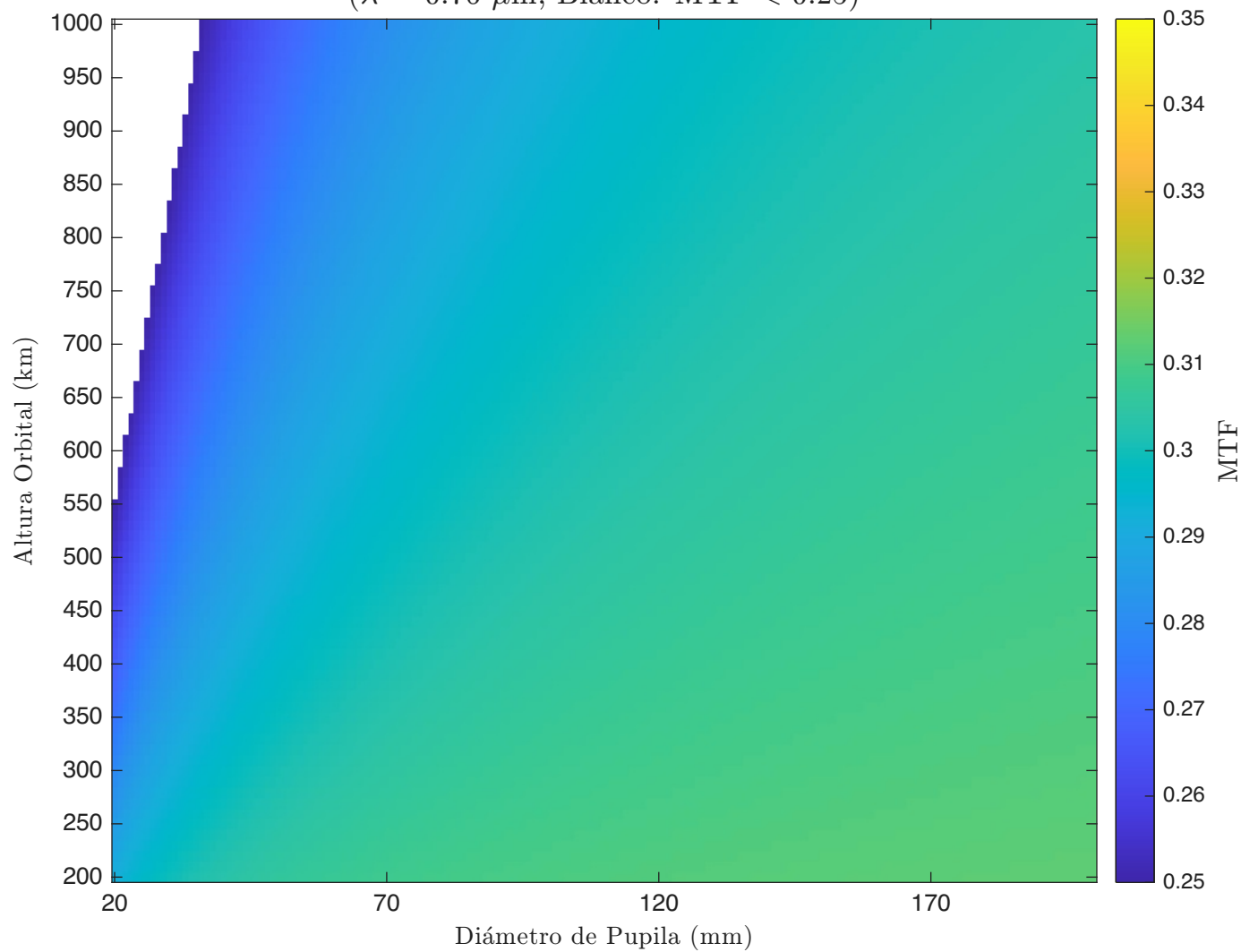
MTF - Cassegrain - Detector 2 ( \lambda = 0.76 \mu\text{m} , Blanco: MTF < 0.25)
